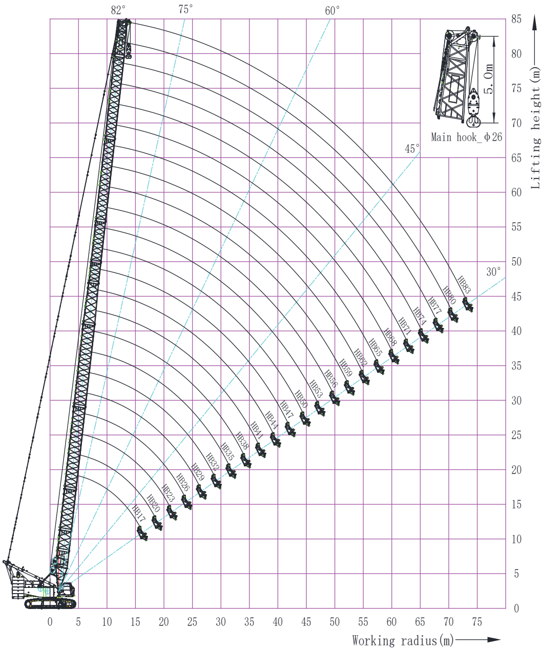
Boom working condition _ boom main hook working range (without boom single top, HB/1)
